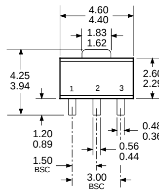
Dwg. MA-009-3A in
