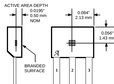
Dwg. MH-011-3D
